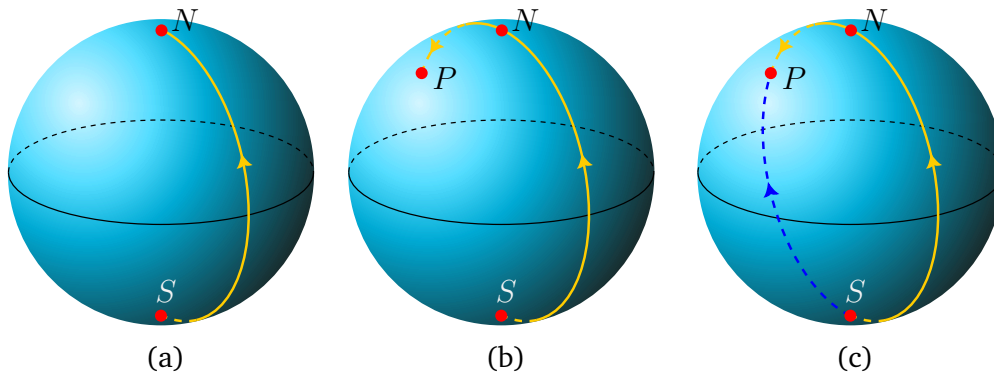
Figure 2.10: Cut locus of south pole in S^2
